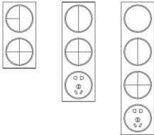
竖排连体 Vertical multi-gang installation
