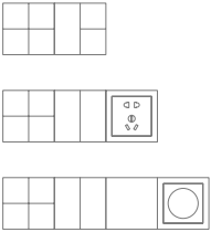
横排连体 Horizontal multi-gang installation
